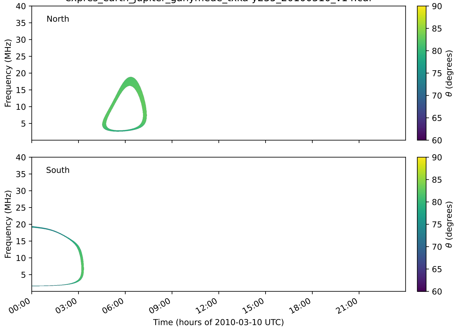
expres_earth_jupiter_ganymede_txka-y235_20100310_v14.cdf
