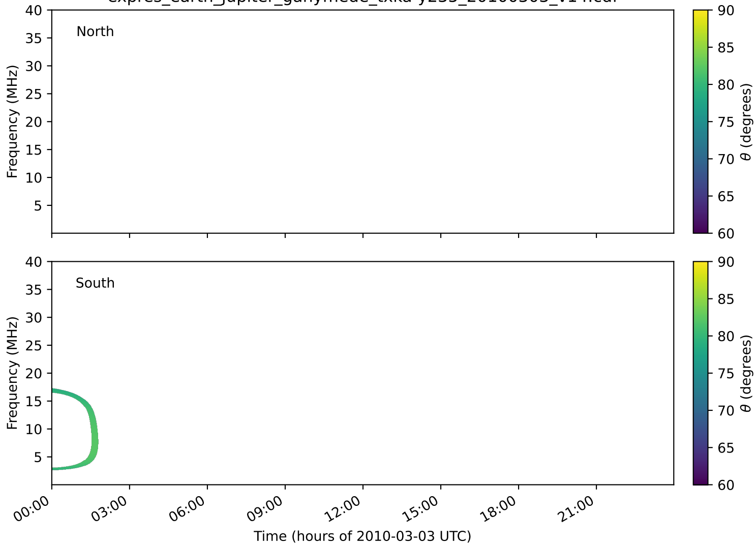
expres_earth_jupiter_ganymede_txka-y235_20100303_v14.cdf
