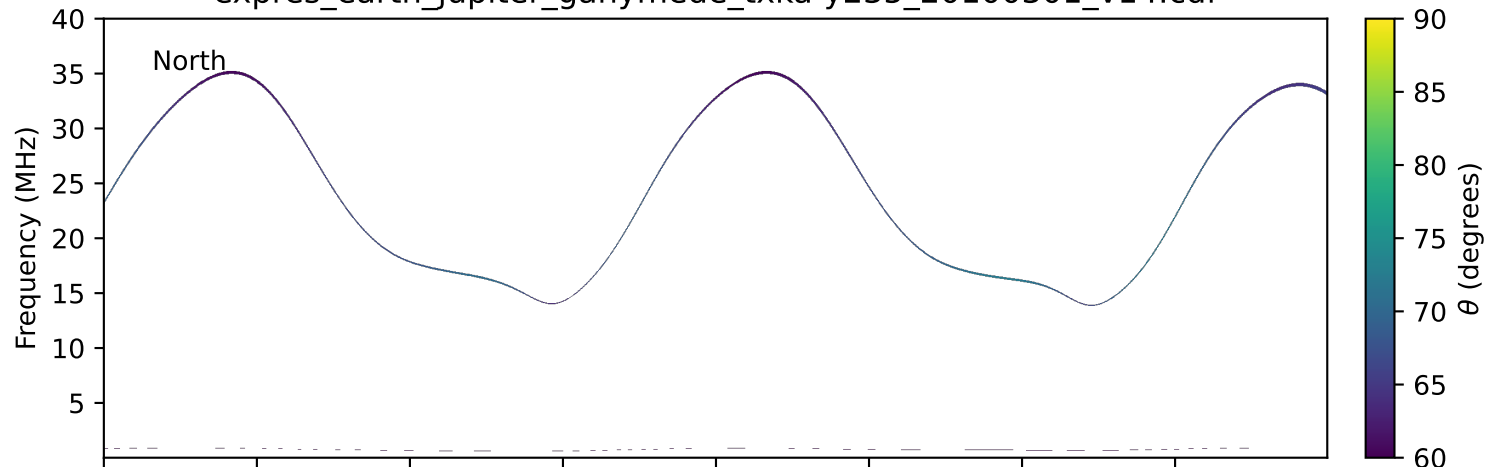
expres_earth_jupiter_ganymede_txka-y235_20100301_v14.cdf
