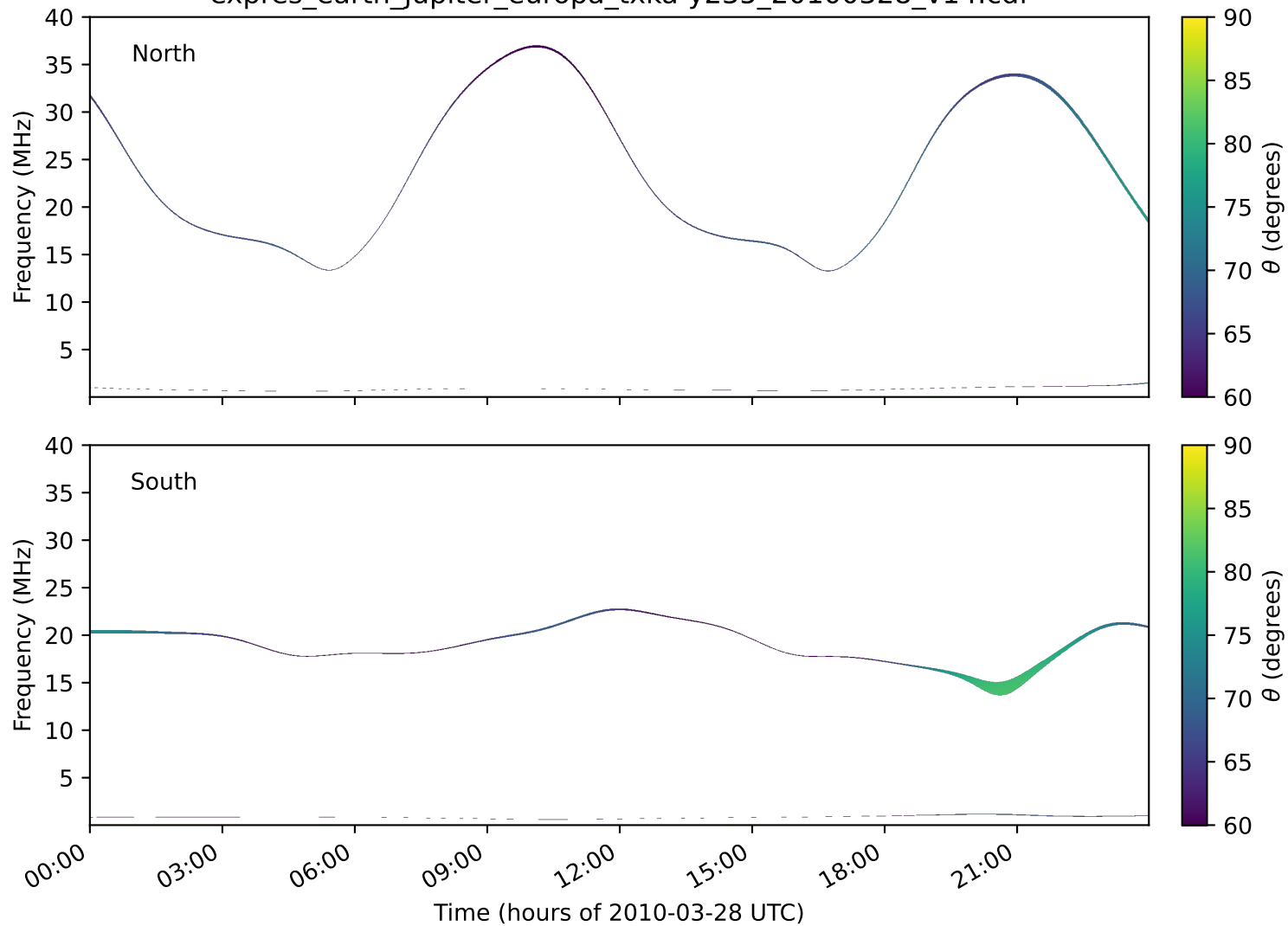
expres_earth_jupiter_europa_txka-y235_20100328_v14.cdf
