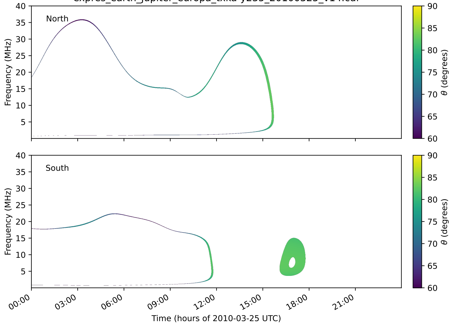
expres_earth_jupiter_europa_txka-y235_20100325_v14.cdf
