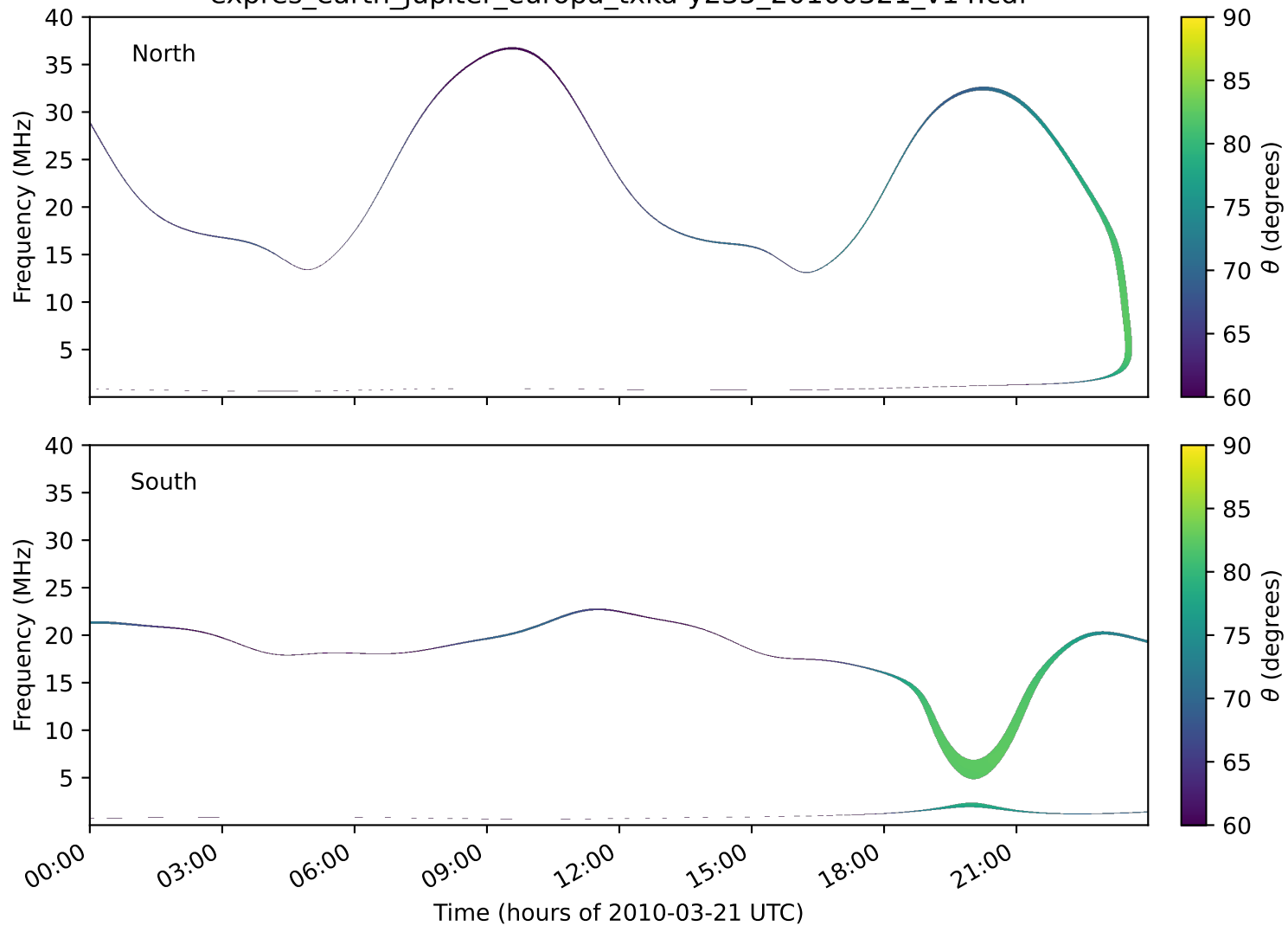
expres_earth_jupiter_europa_txka-y235_20100321_v14.cdf
