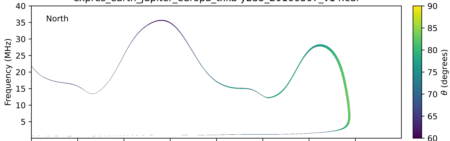
expres_earth_jupiter_europa_txka-y235_20100307_v14.cdf
