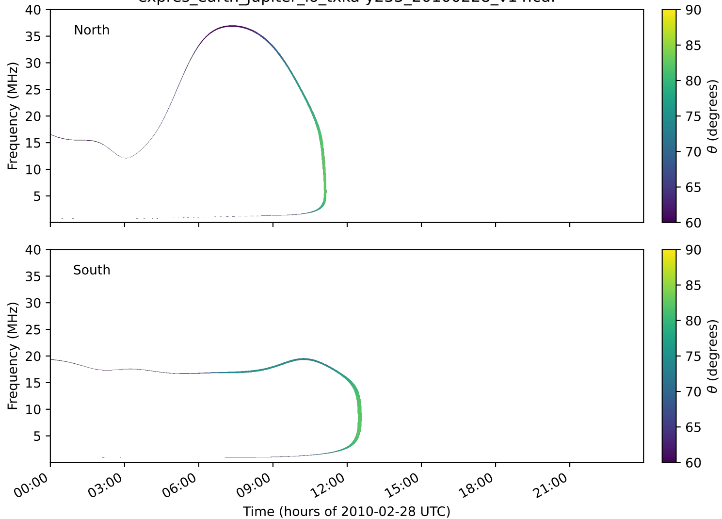
expres_earth_jupiter_io_txka-y235_20100228_v14.cdf
