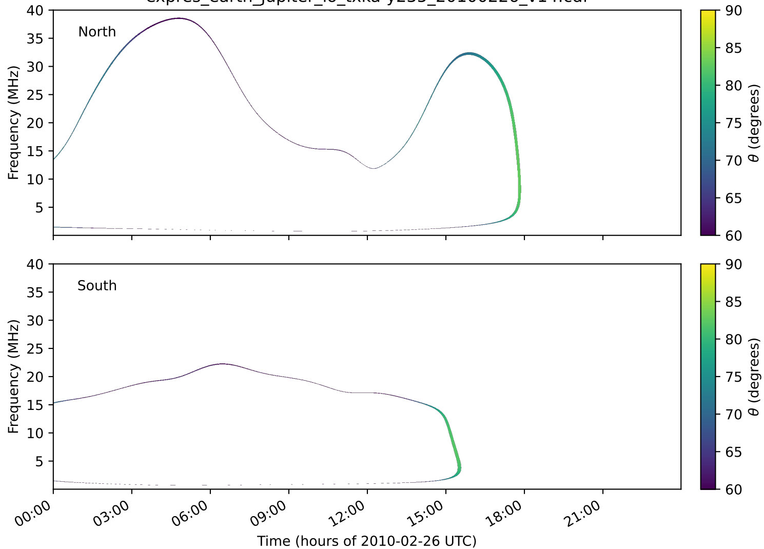
expres_earth_jupiter_io_txka-y235_20100226_v14.cdf
