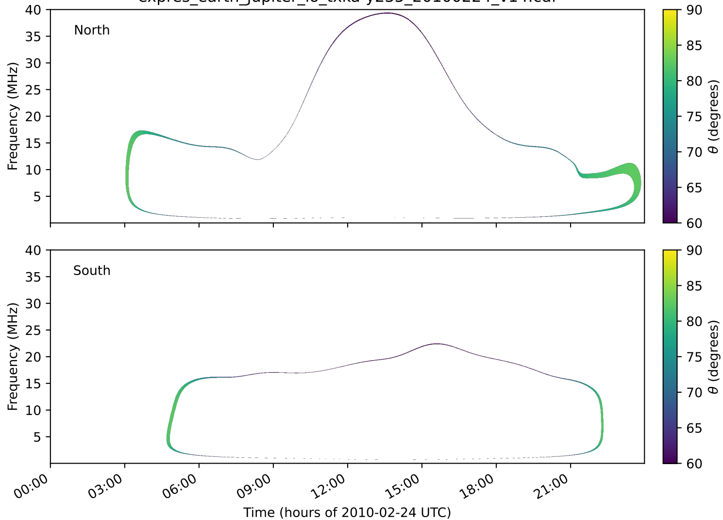
expres_earth_jupiter_io_txka-y235_20100224_v14.cdf
