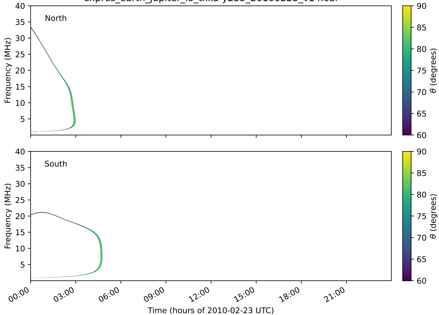
expres_earth_jupiter_io_txka-y235_20100223_v14.cdf
