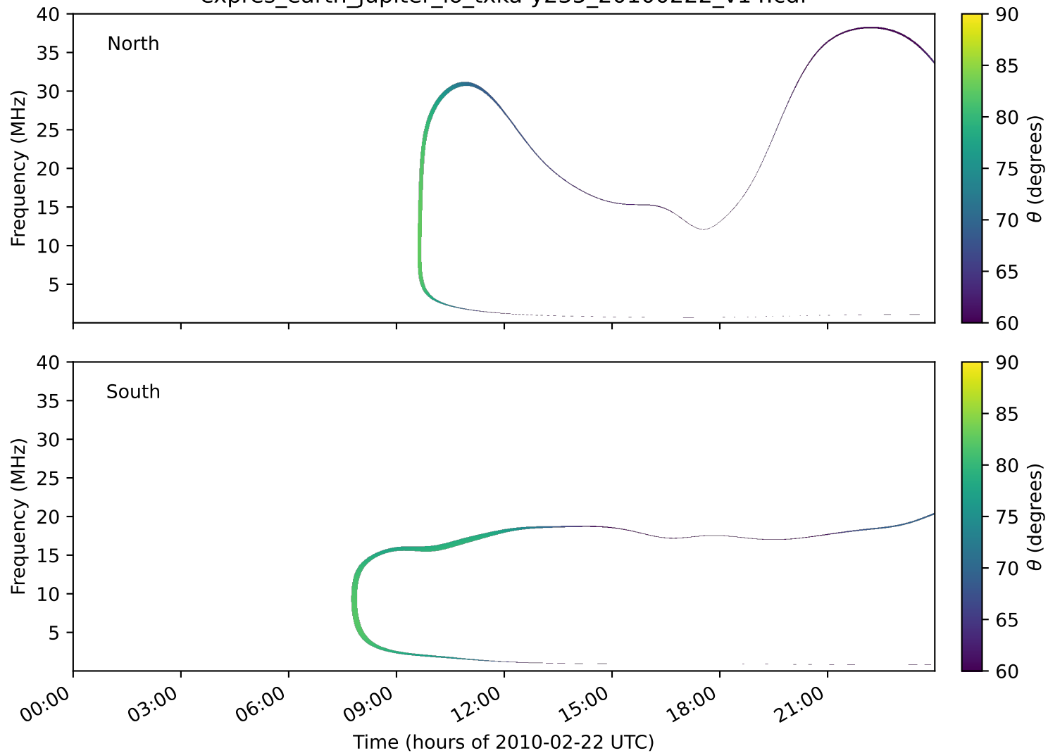
expres_earth_jupiter_io_txka-y235_20100222_v14.cdf
