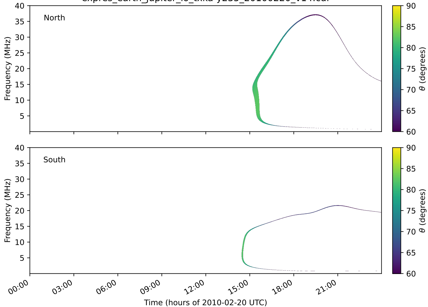
expres_earth_jupiter_io_txka-y235_20100220_v14.cdf
