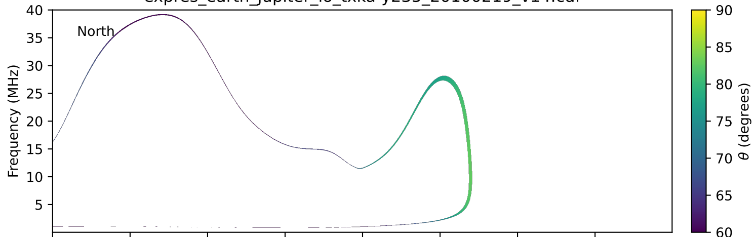
expres_earth_jupiter_io_txka-y235_20100219_v14.cdf
