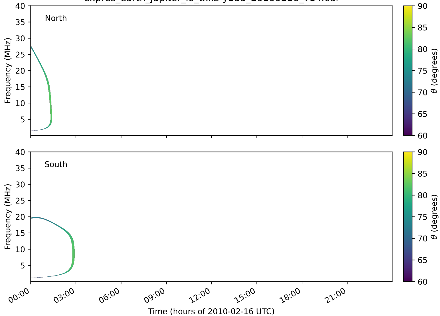
expres_earth_jupiter_io_txka-y235_20100216_v14.cdf
