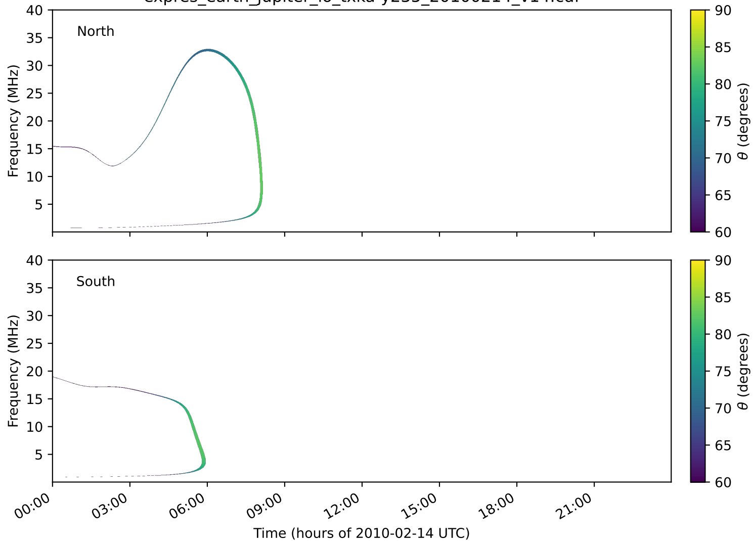
expres_earth_jupiter_io_txka-y235_20100214_v14.cdf
