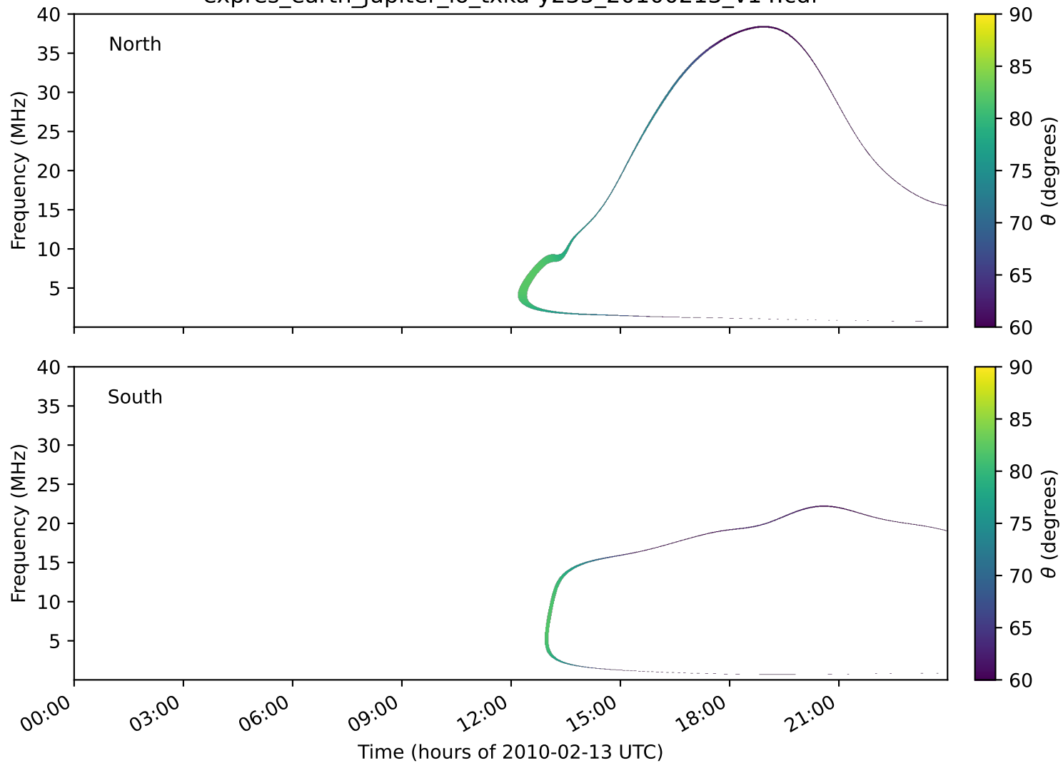
expres_earth_jupiter_io_txka-y235_20100213_v14.cdf
