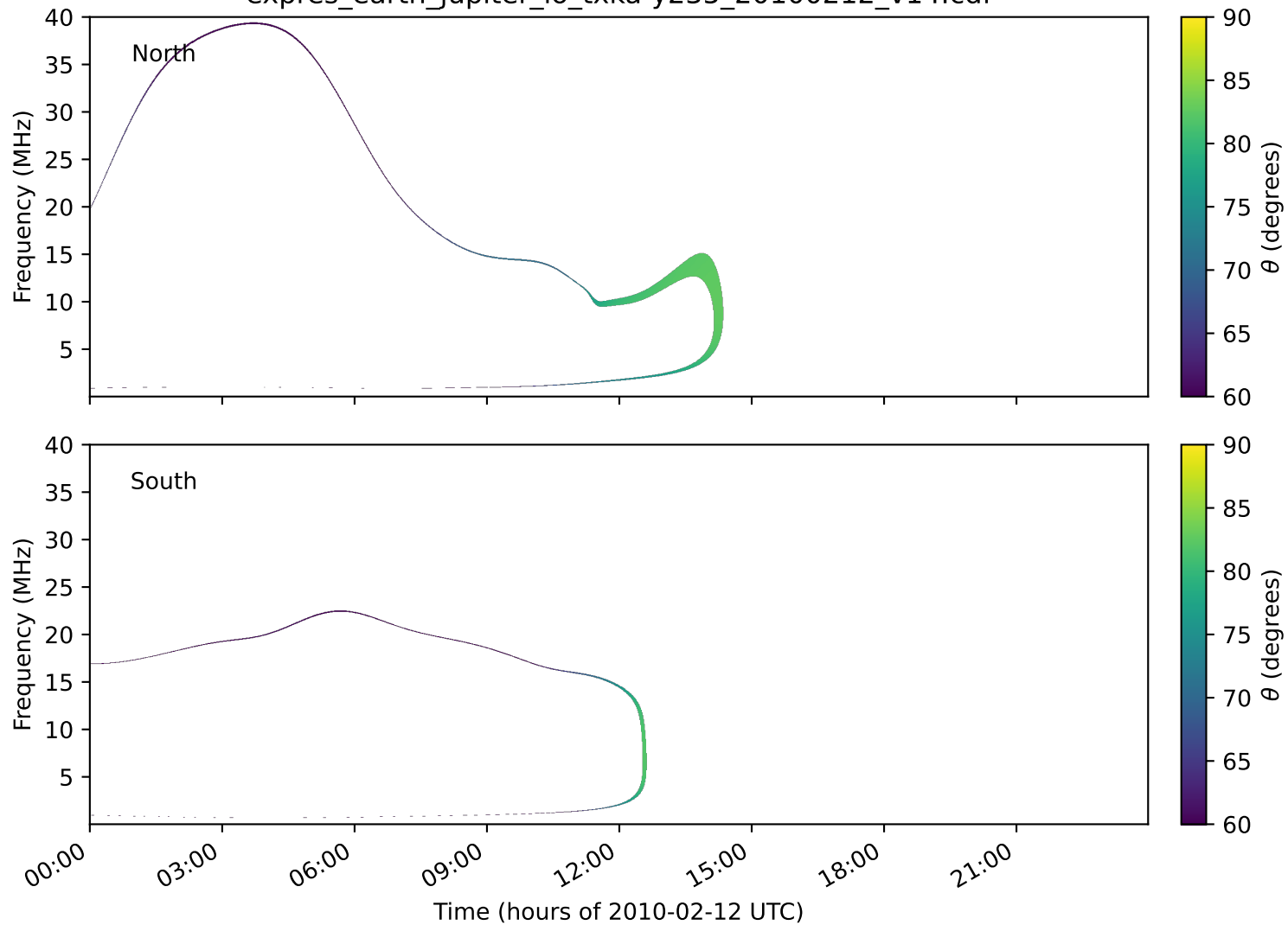
expres_earth_jupiter_io_txka-y235_20100212_v14.cdf
