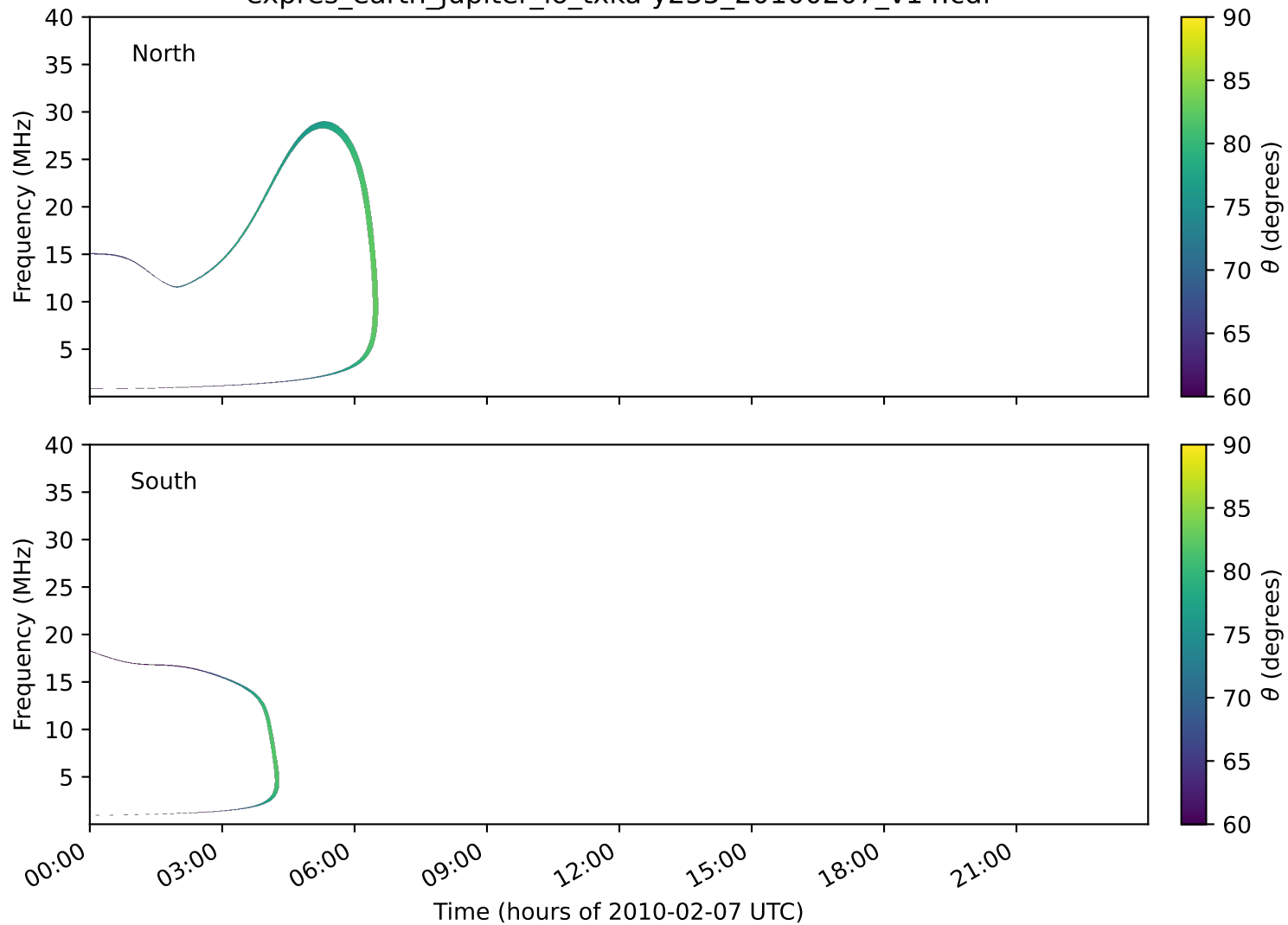
expres_earth_jupiter_io_txka-y235_20100207_v14.cdf
