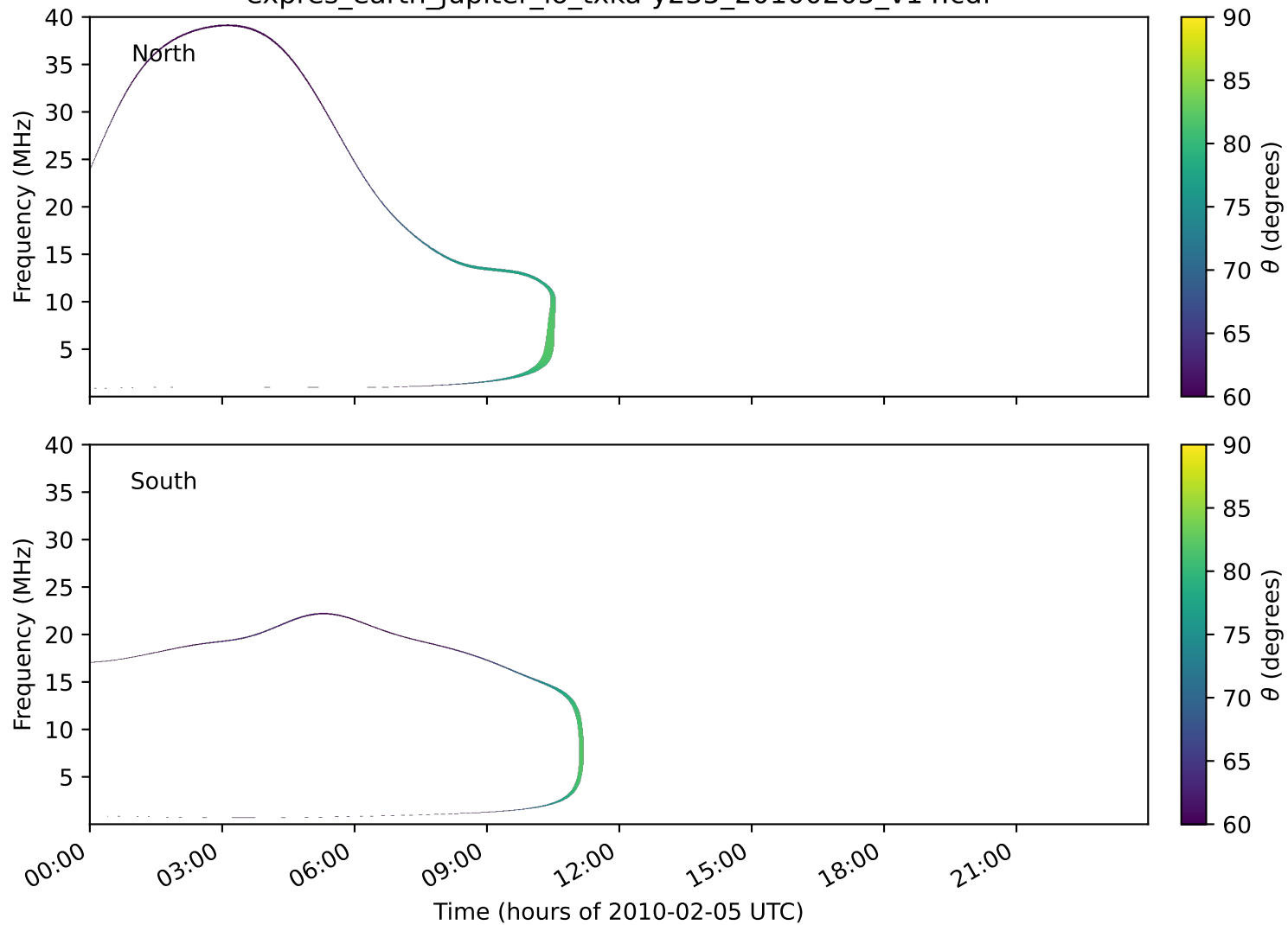
expres_earth_jupiter_io_txka-y235_20100205_v14.cdf
