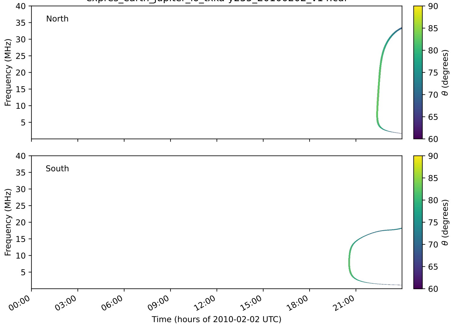
expres_earth_jupiter_io_txka-y235_20100202_v14.cdf
