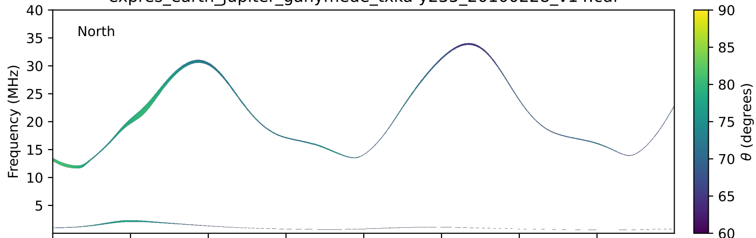
expres_earth_jupiter_ganymede_txka-y235_20100228_v14.cdf
