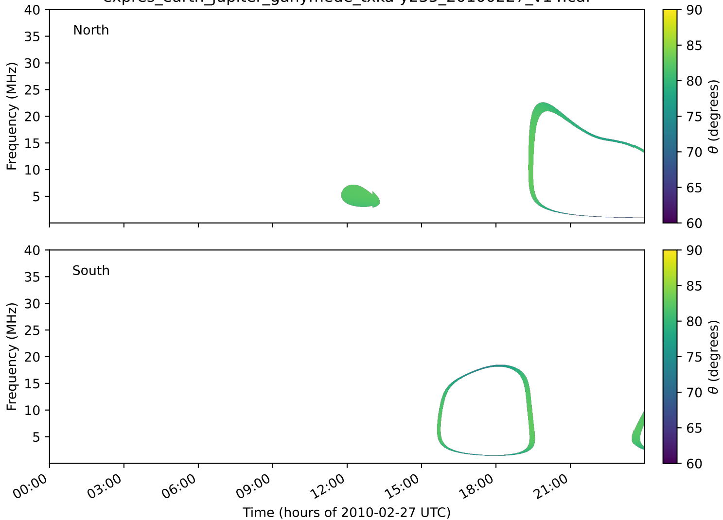
expres_earth_jupiter_ganymede_txka-y235_20100227_v14.cdf
