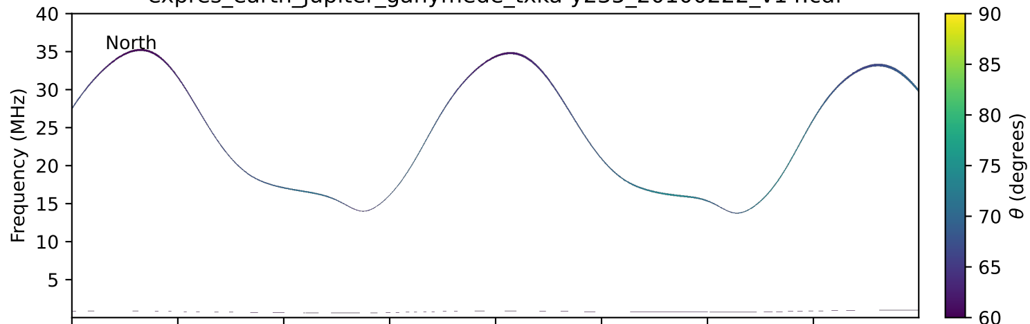
expres_earth_jupiter_ganymede_txka-y235_20100222_v14.cdf
