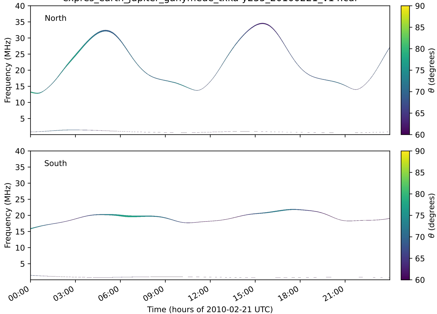
expres_earth_jupiter_ganymede_txka-y235_20100221_v14.cdf
