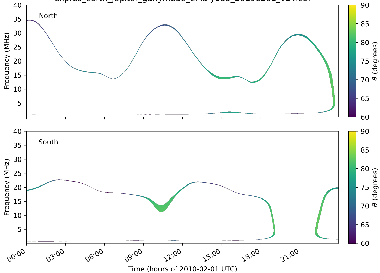
expres_earth_jupiter_ganymede_txka-y235_20100201_v14.cdf
