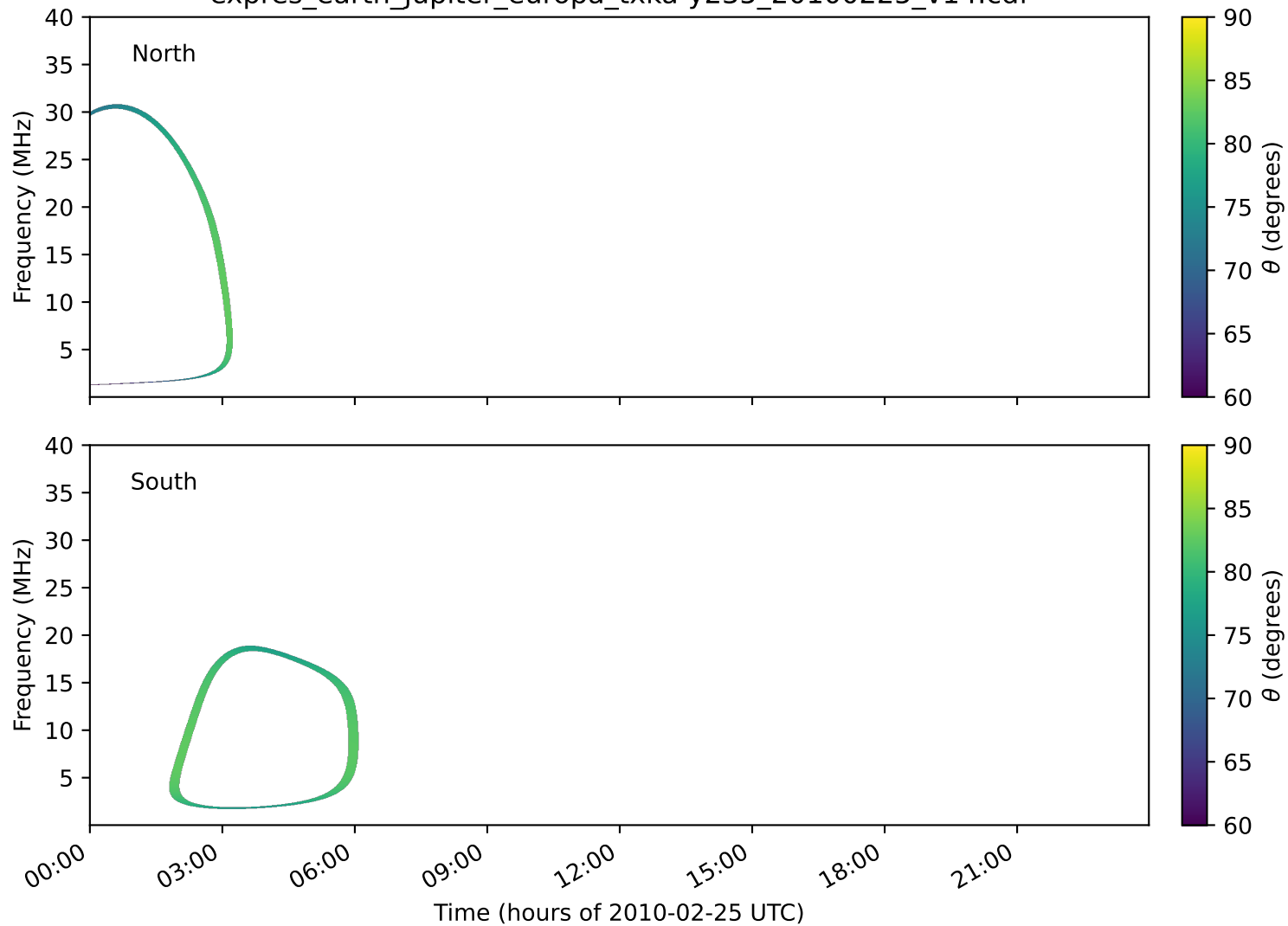
expres_earth_jupiter_europa_txka-y235_20100225_v14.cdf
