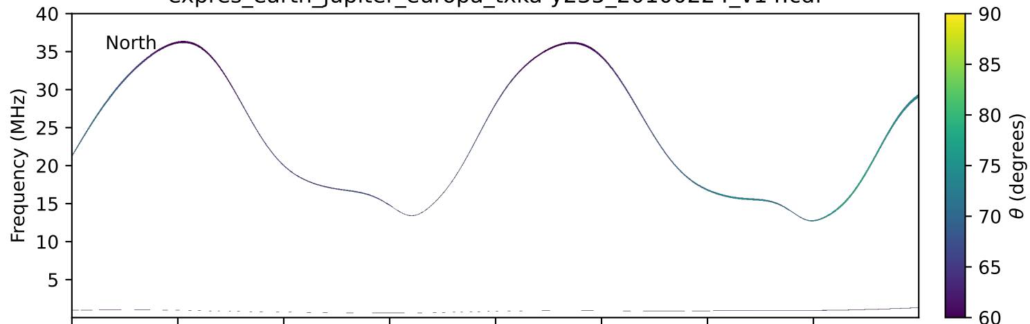
expres_earth_jupiter_europa_txka-y235_20100224_v14.cdf
