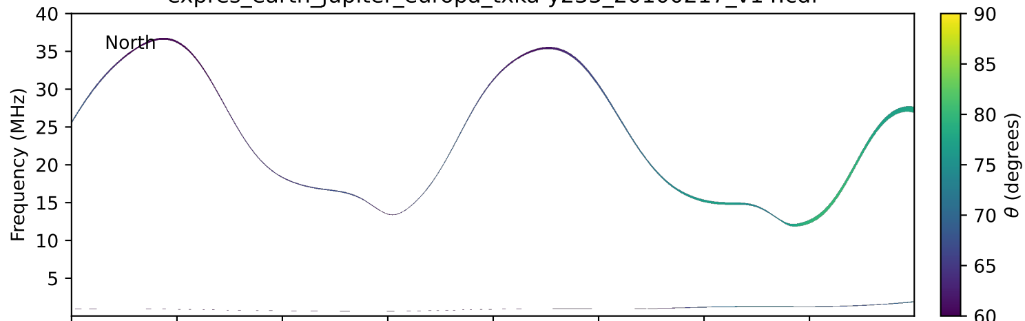
expres_earth_jupiter_europa_txka-y235_20100217_v14.cdf
