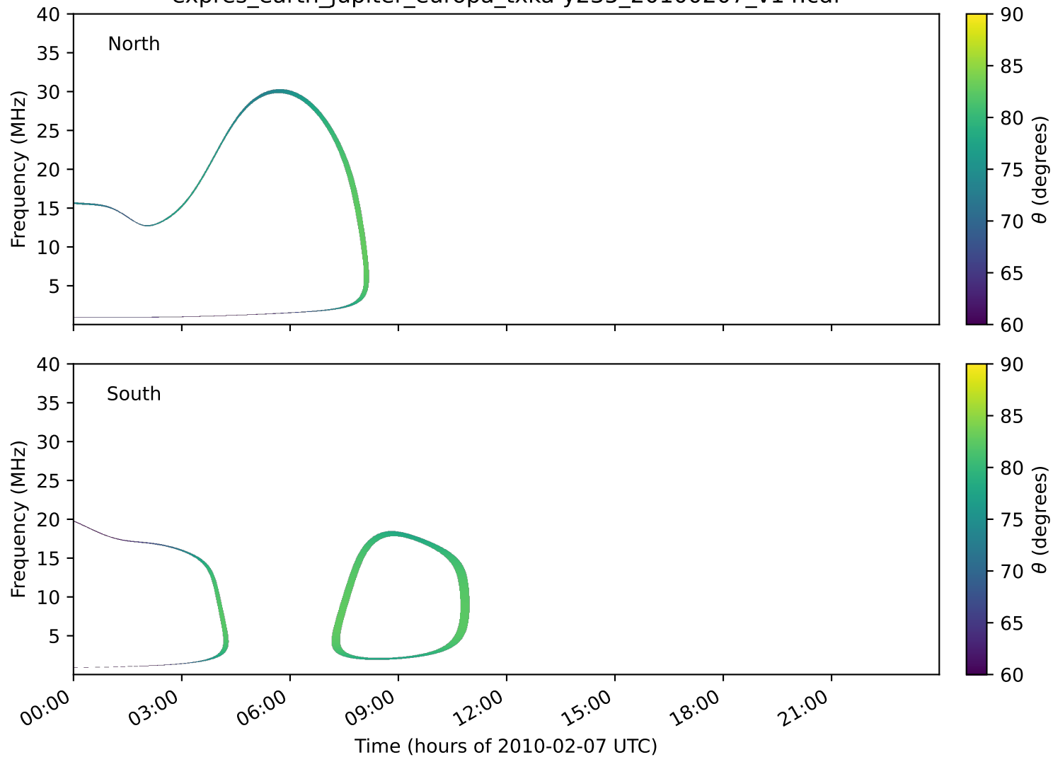
expres_earth_jupiter_europa_txka-y235_20100207_v14.cdf
