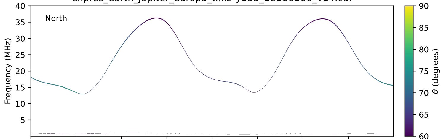
expres_earth_jupiter_europa_txka-y235_20100206_v14.cdf
