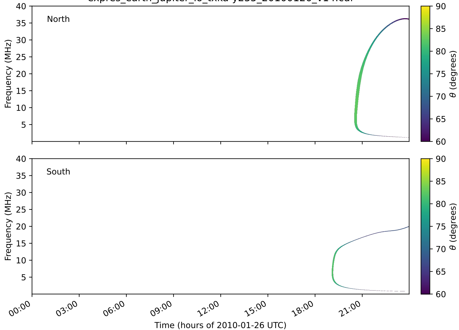
expres_earth_jupiter_io_txka-y235_20100126_v14.cdf
