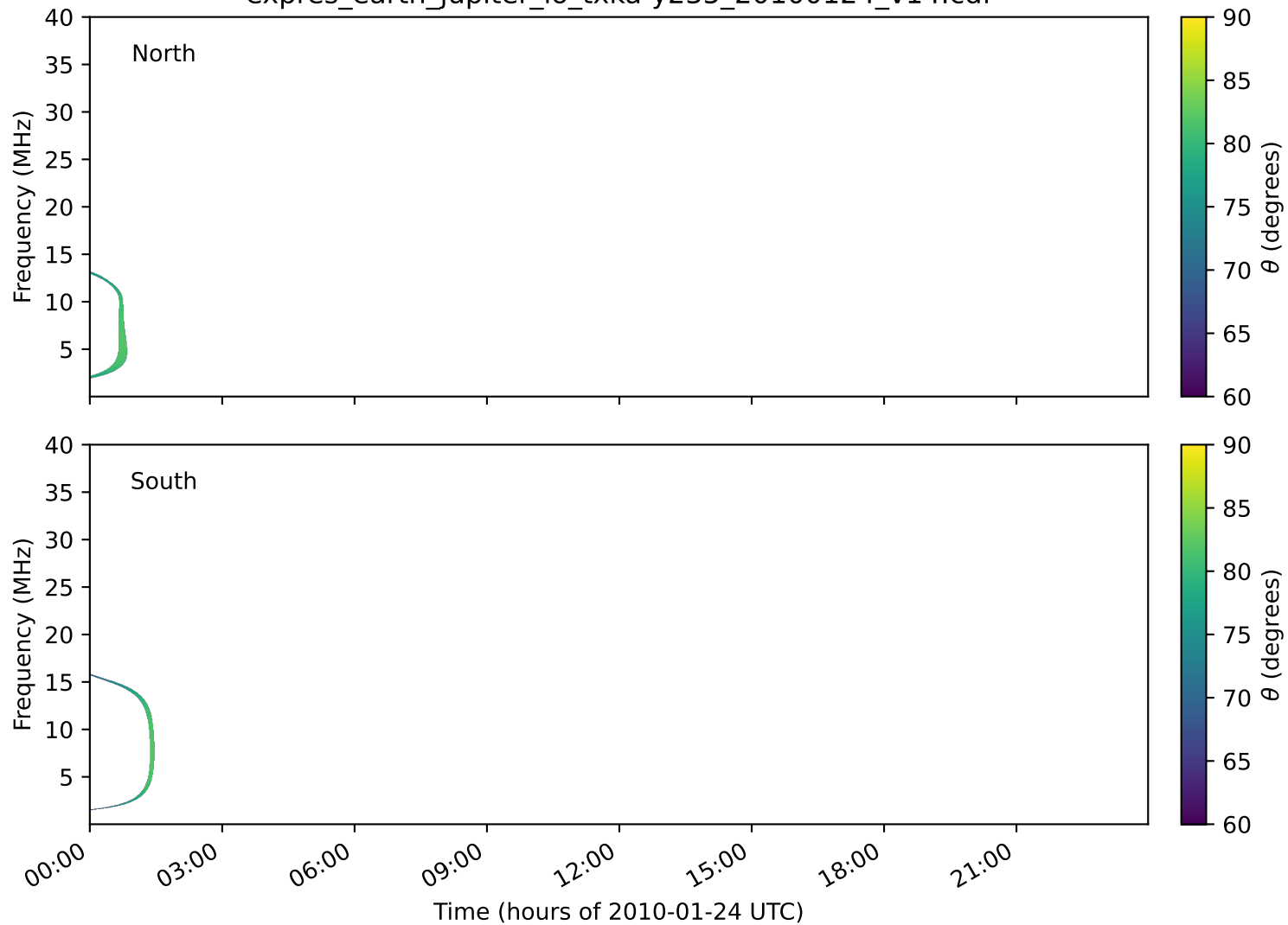
expres_earth_jupiter_io_txka-y235_20100124_v14.cdf
