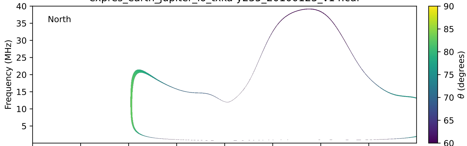
expres_earth_jupiter_io_txka-y235_20100123_v14.cdf
