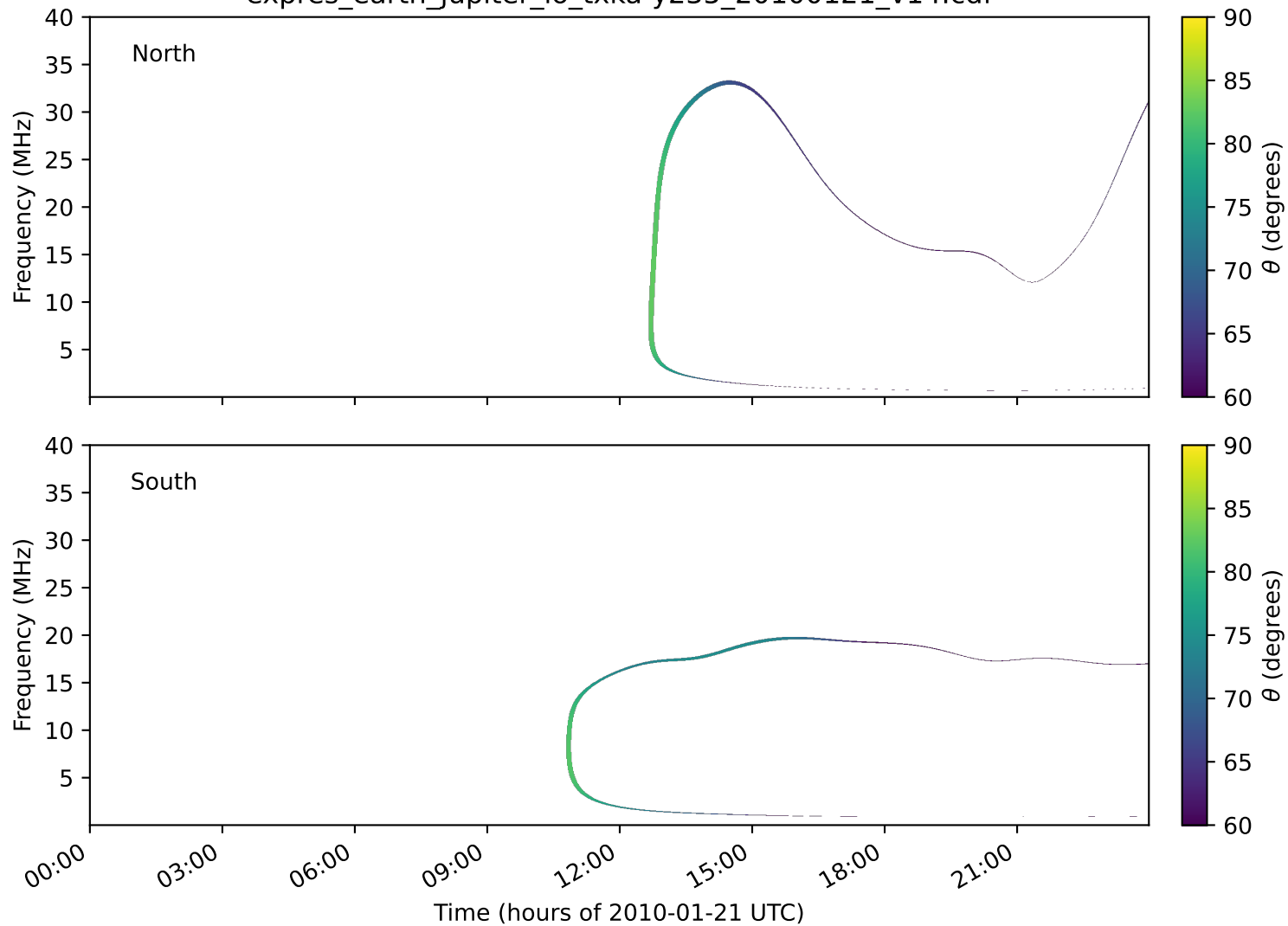
expres_earth_jupiter_io_txka-y235_20100121_v14.cdf
