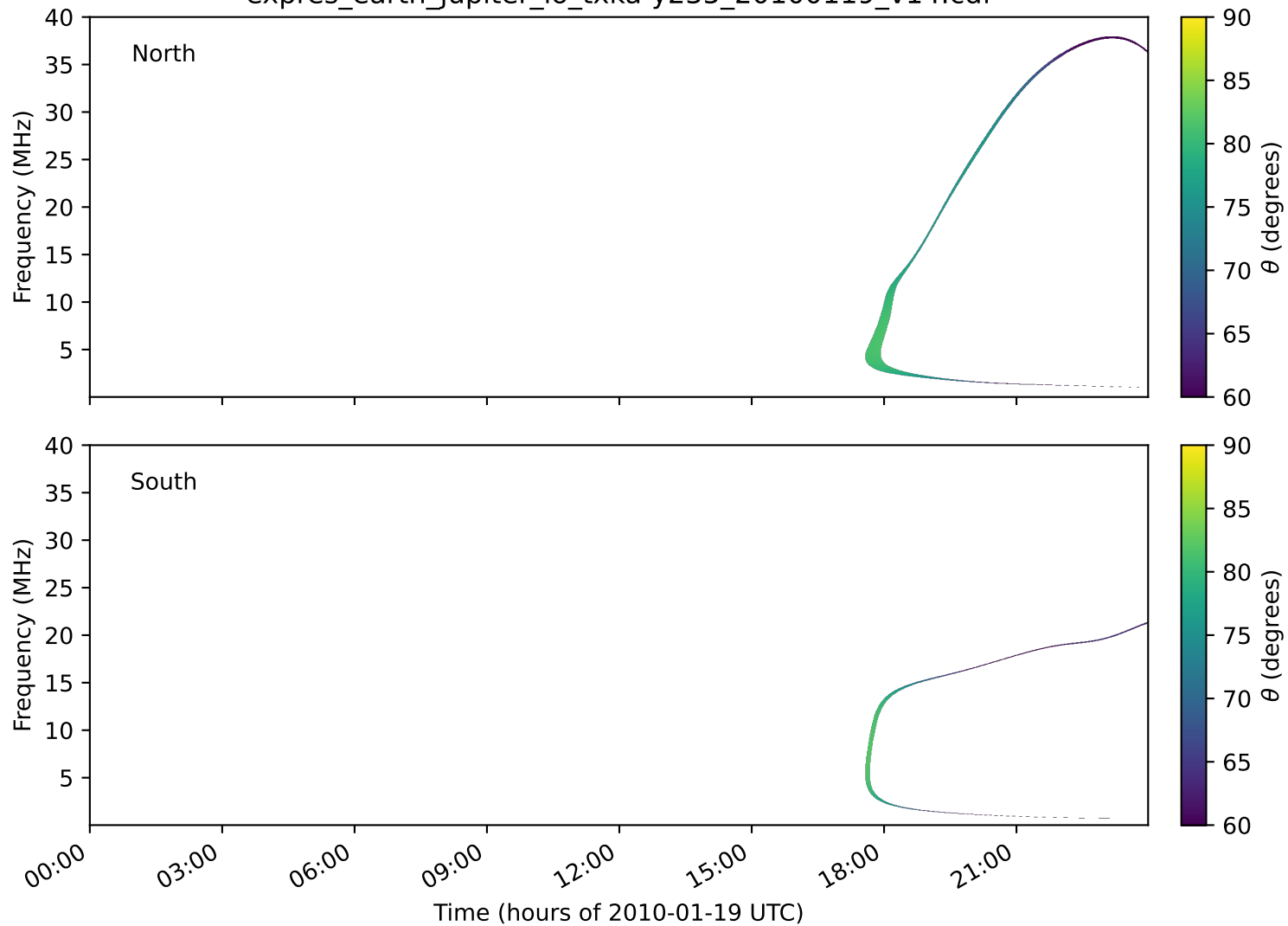
expres_earth_jupiter_io_txka-y235_20100119_v14.cdf
