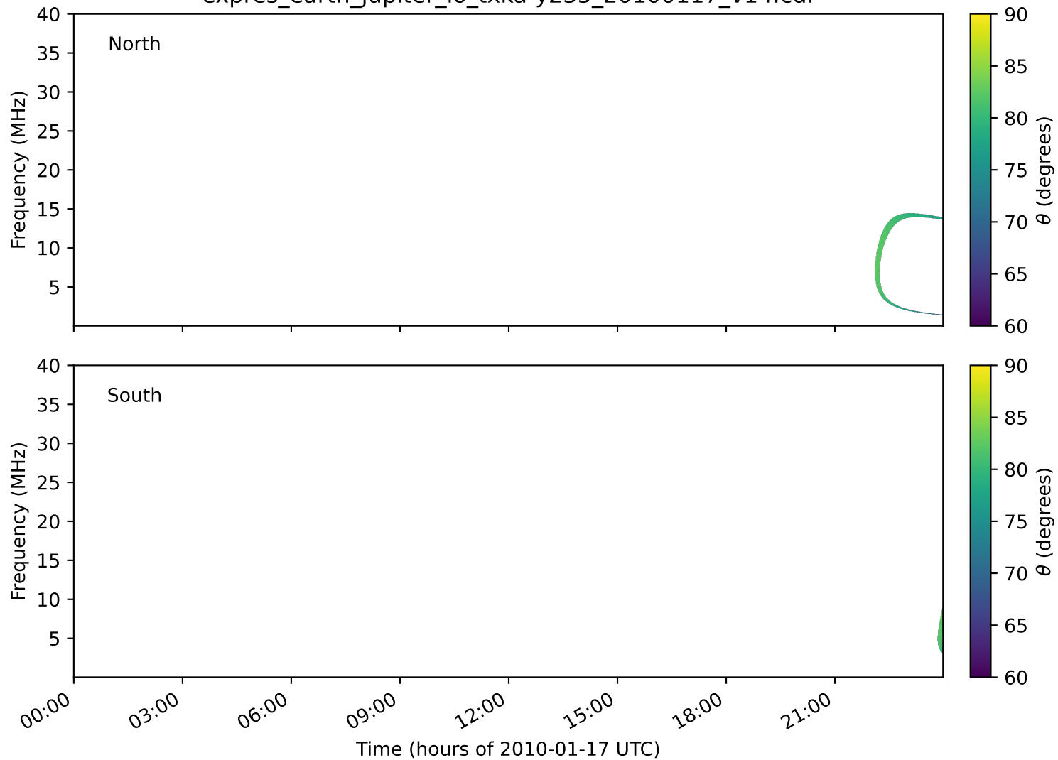
expres_earth_jupiter_io_txka-y235_20100117_v14.cdf
