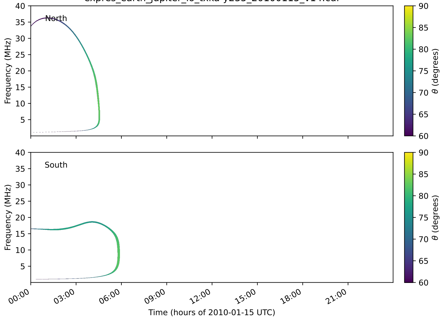
expres_earth_jupiter_io_txka-y235_20100115_v14.cdf
