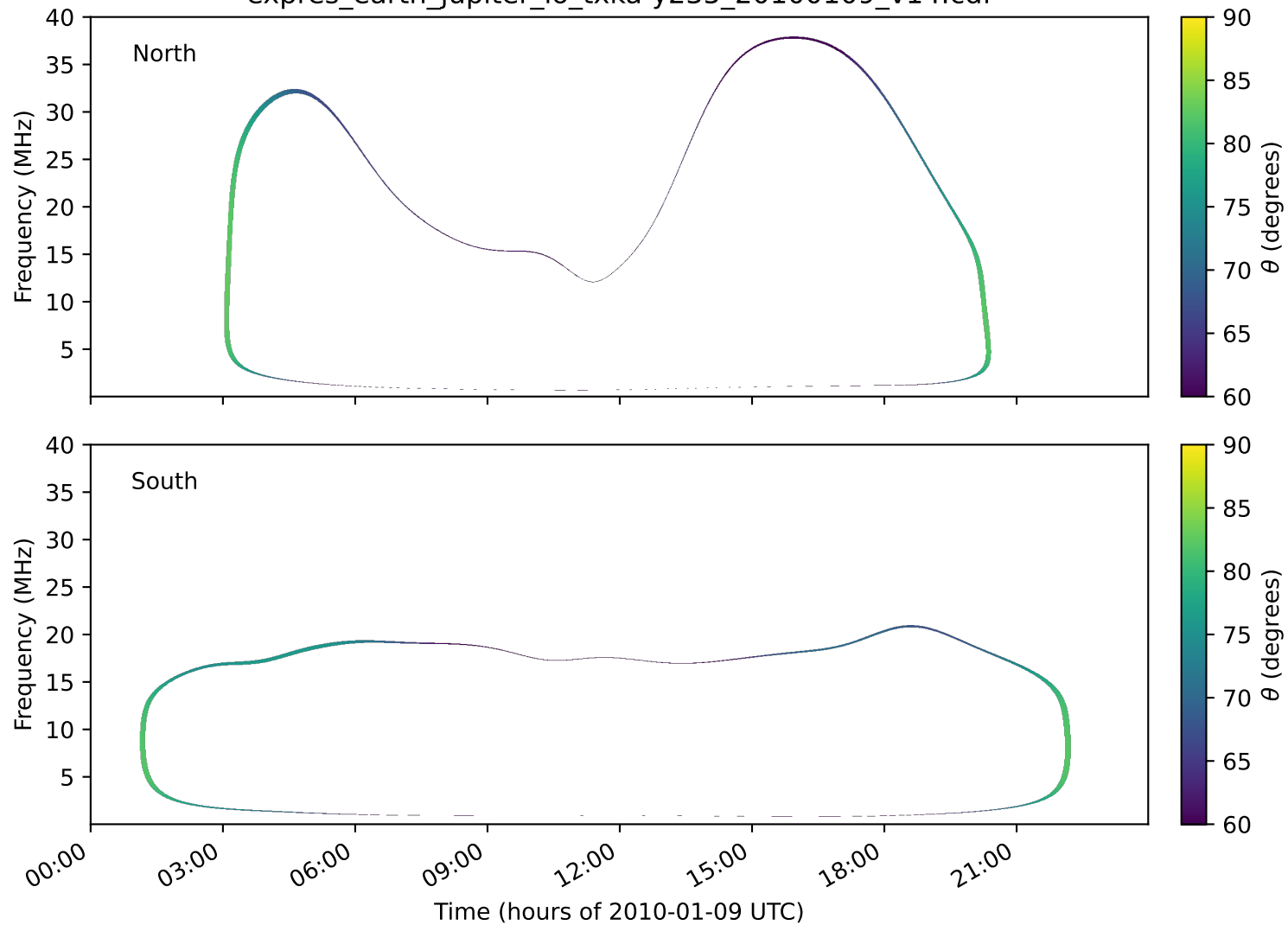
expres_earth_jupiter_io_txka-y235_20100109_v14.cdf
