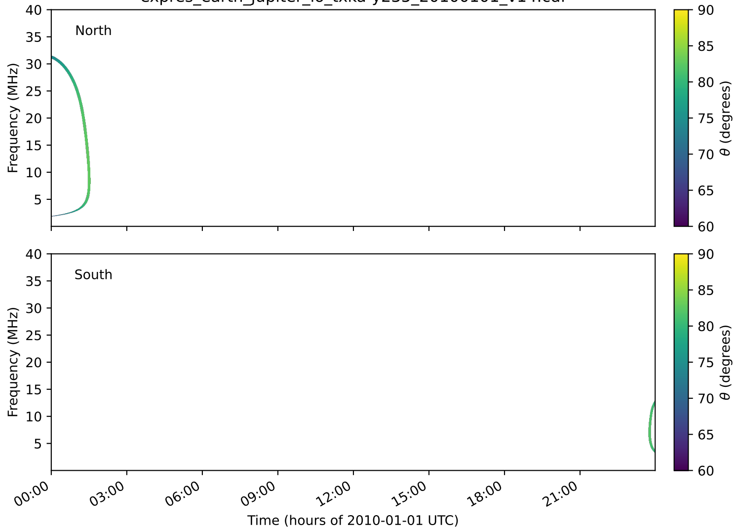
expres_earth_jupiter_io_txka-y235_20100101_v14.cdf
