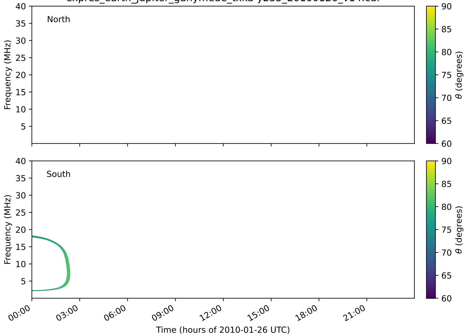
expres_earth_jupiter_ganymede_txka-y235_20100126_v14.cdf
