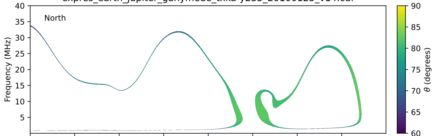
expres_earth_jupiter_ganymede_txka-y235_20100125_v14.cdf
