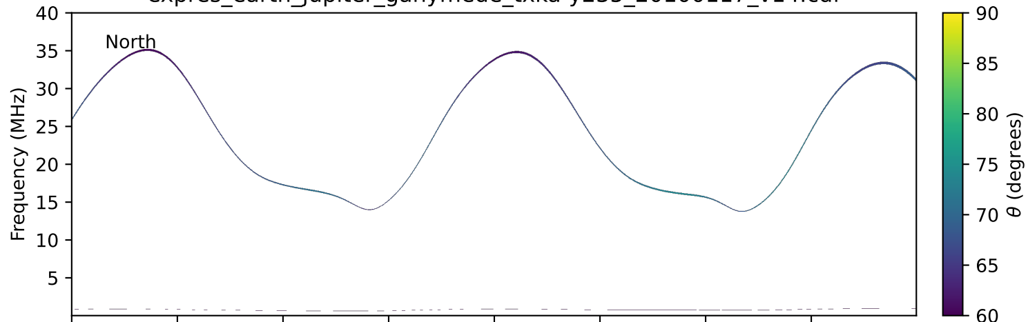
expres_earth_jupiter_ganymede_txka-y235_20100117_v14.cdf
