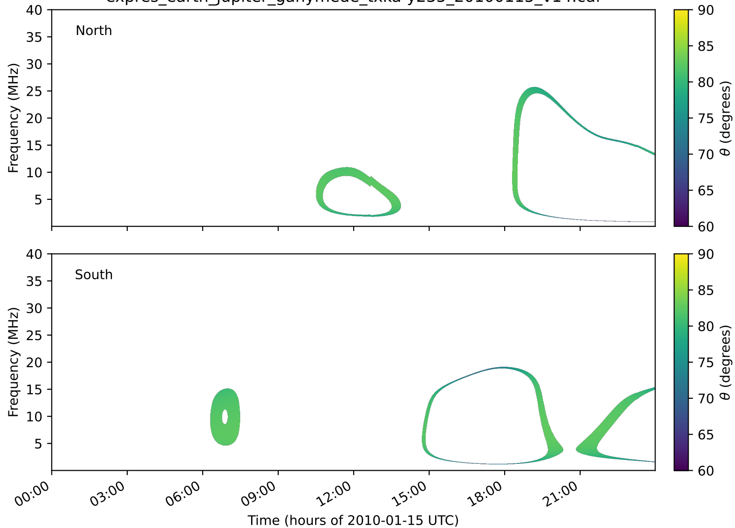
expres_earth_jupiter_ganymede_txka-y235_20100115_v14.cdf
