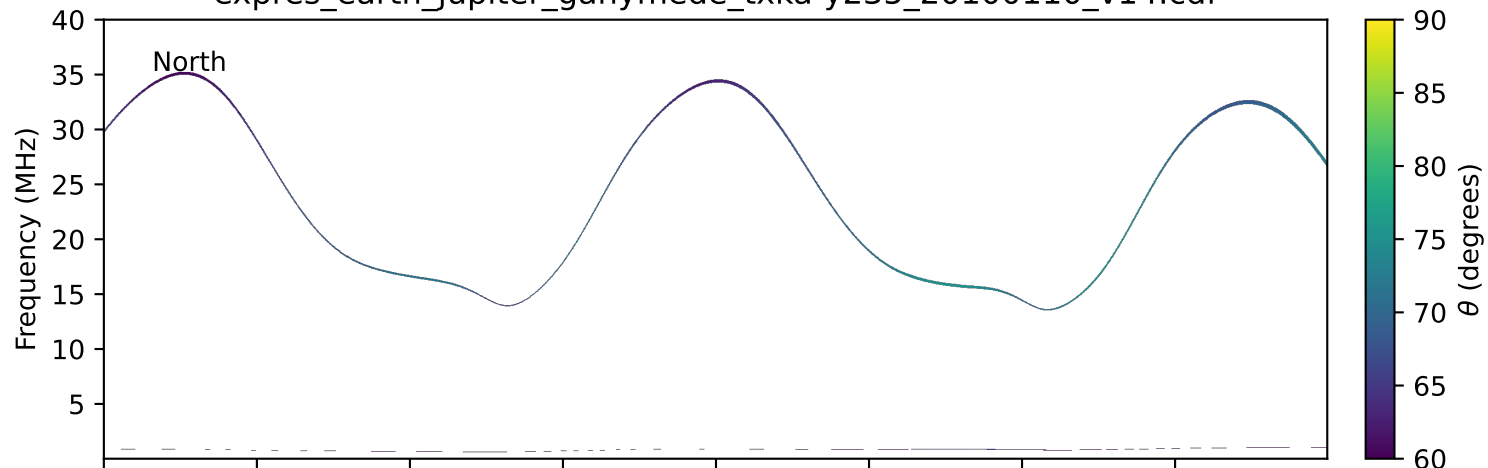
expres_earth_jupiter_ganymede_txka-y235_20100110_v14.cdf
