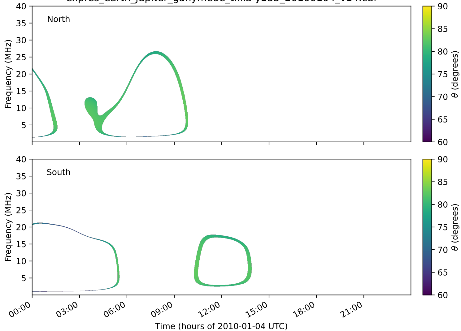
expres_earth_jupiter_ganymede_txka-y235_20100104_v14.cdf
