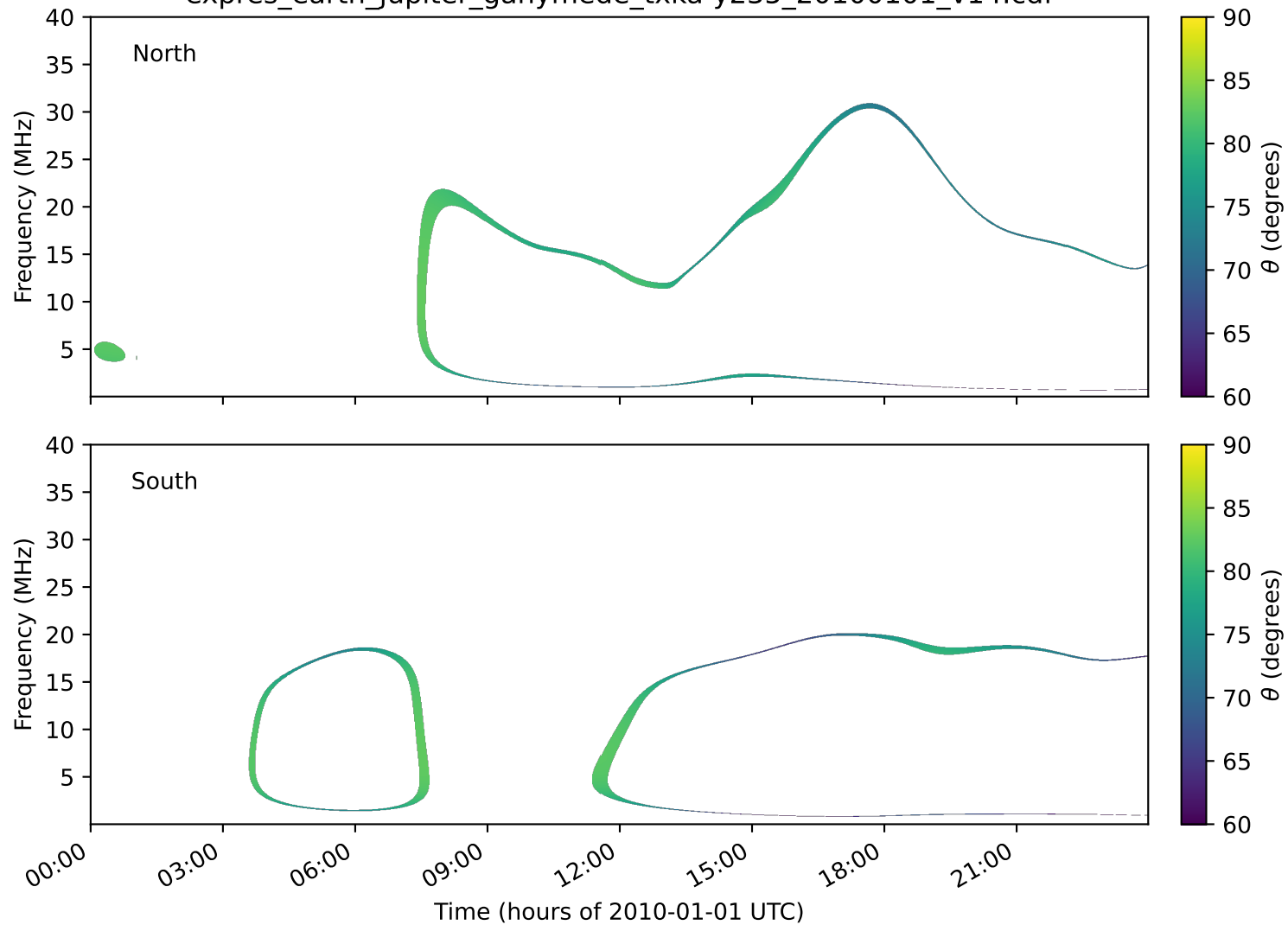
expres_earth_jupiter_ganymede_txka-y235_20100101_v14.cdf
