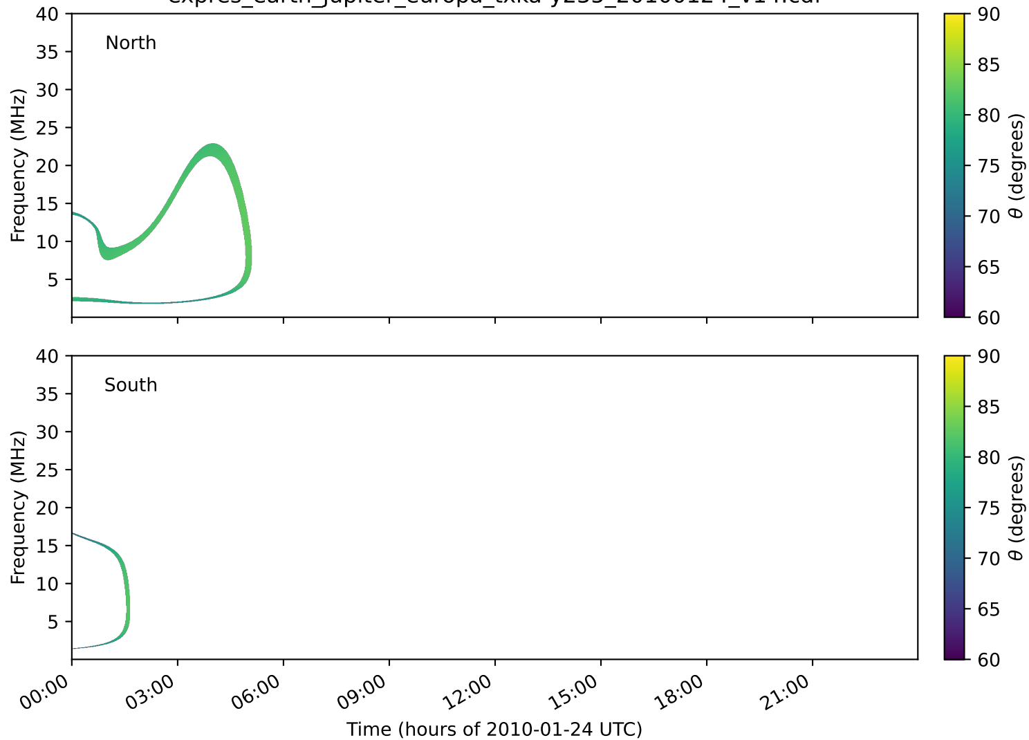
expres_earth_jupiter_europa_txka-y235_20100124_v14.cdf
