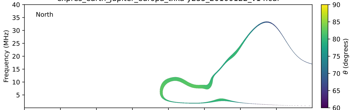
expres_earth_jupiter_europa_txka-y235_20100122_v14.cdf
