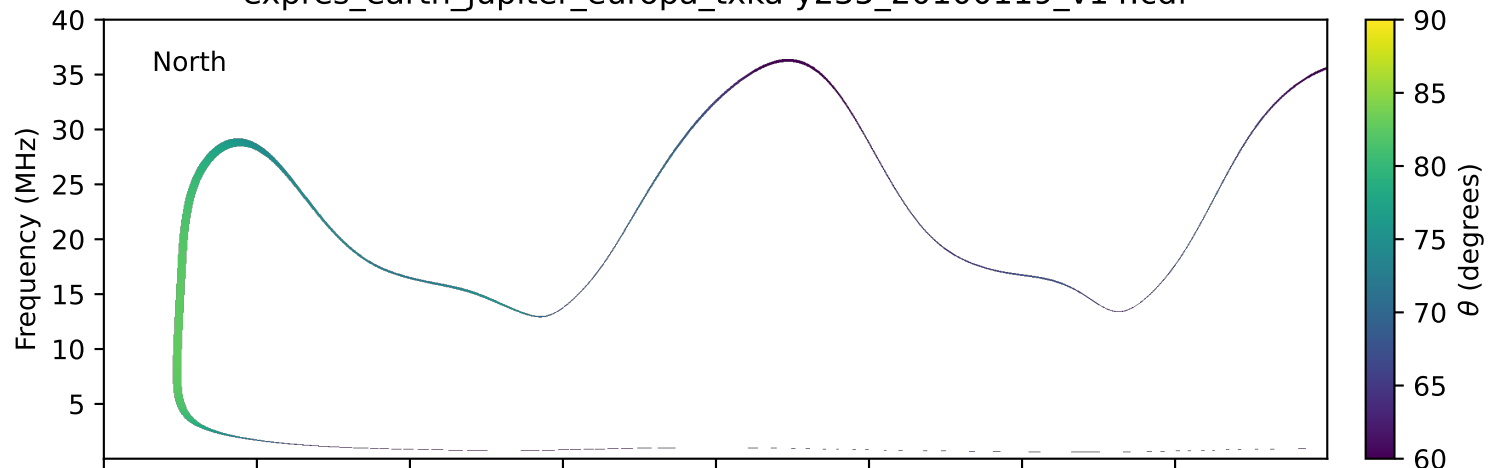
expres_earth_jupiter_europa_txka-y235_20100119_v14.cdf
